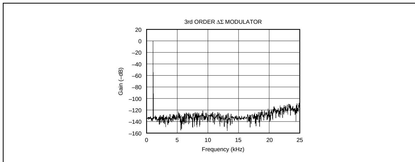
FIGURE 17. Quantization Noise Spectrum.
